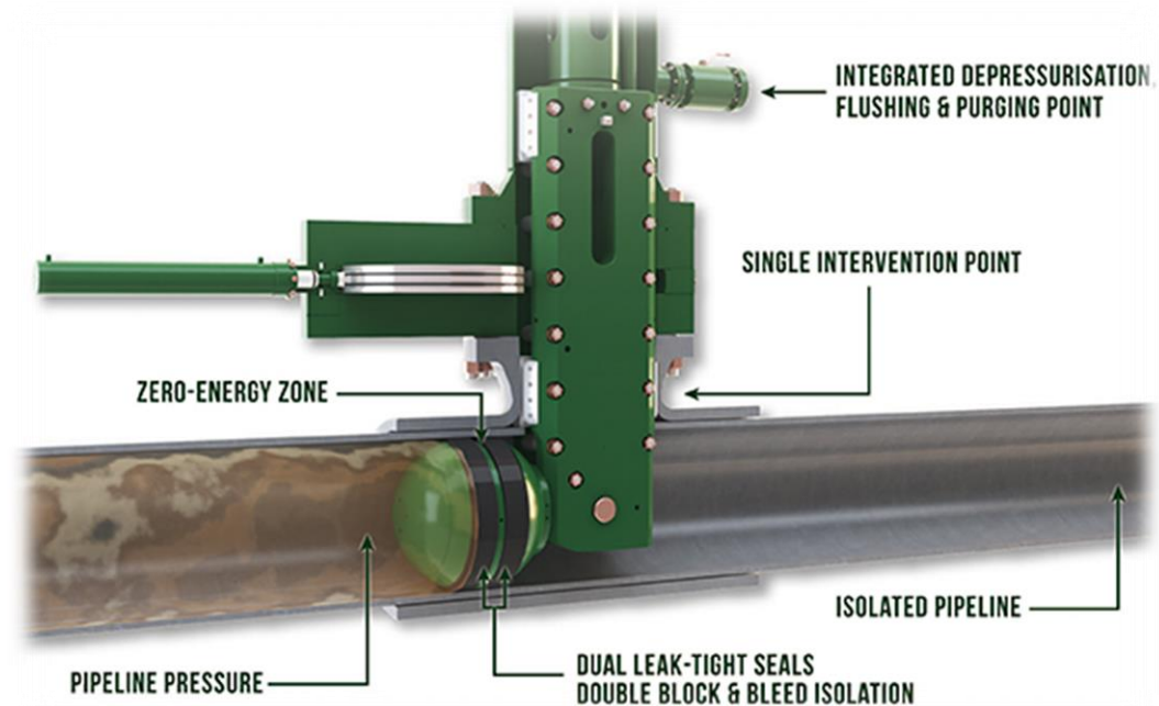
Standard BISEP® Deployment
