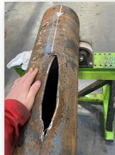
9 5/8" Perforation
